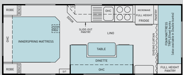
G2-206X-3B (WITH FRONT BOOT)
