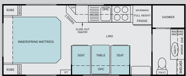
G2-206X-CAF (WITH FRONT BOOT)
